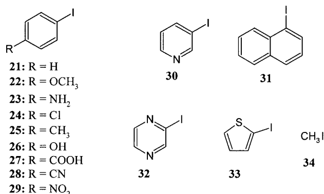
Figure 2. Halides.
