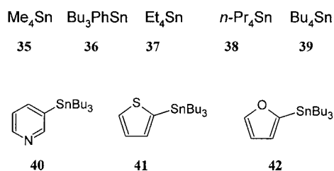
Figure 3. Organostannyl compounds.
